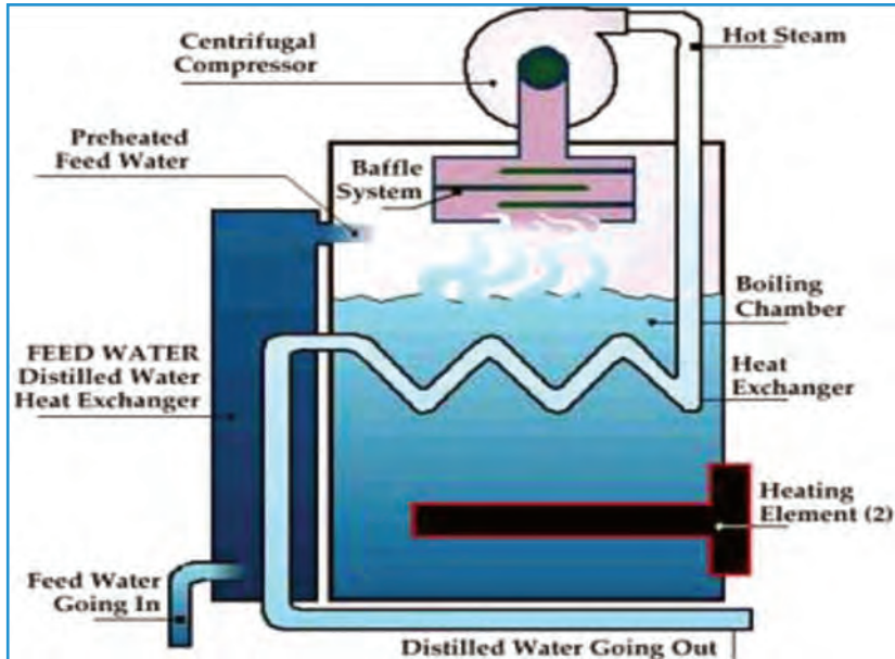
Fig 11.3 - Schematic view of vapour compressor distillation system
