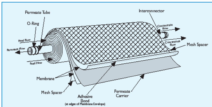
Fig 11.6 - Cut away view of spiral wound membrane element
