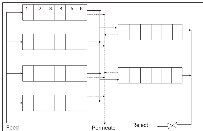
Reject staging
