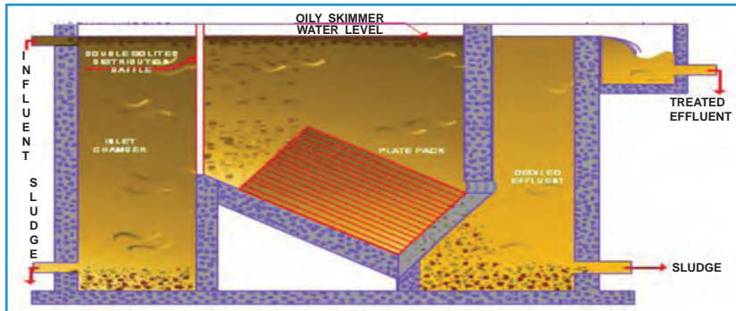
Fig 12.5 - A typical TPI oil separator
