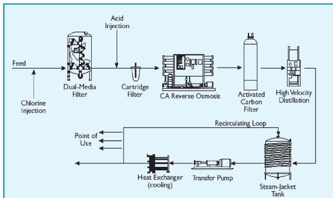
Fig 8.3 – Production of water for injectables
