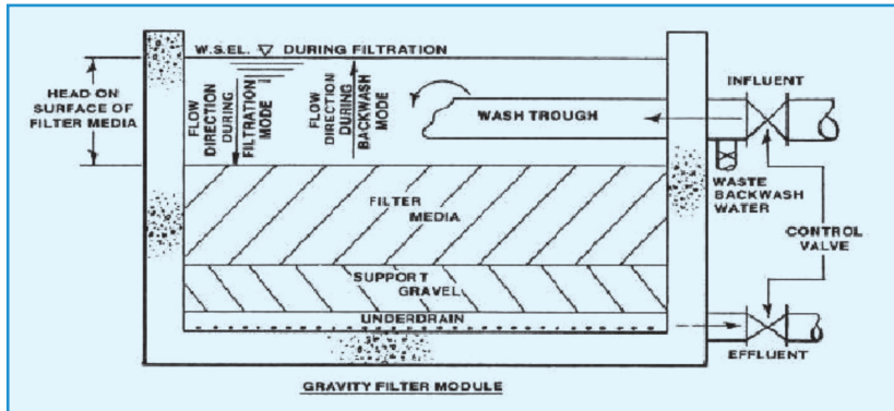
Fig 3.11 - Cross section drawing of rapid gravity sand filter
