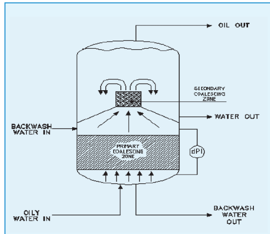
Fig 12.7 - A typical oil coalescer unit
